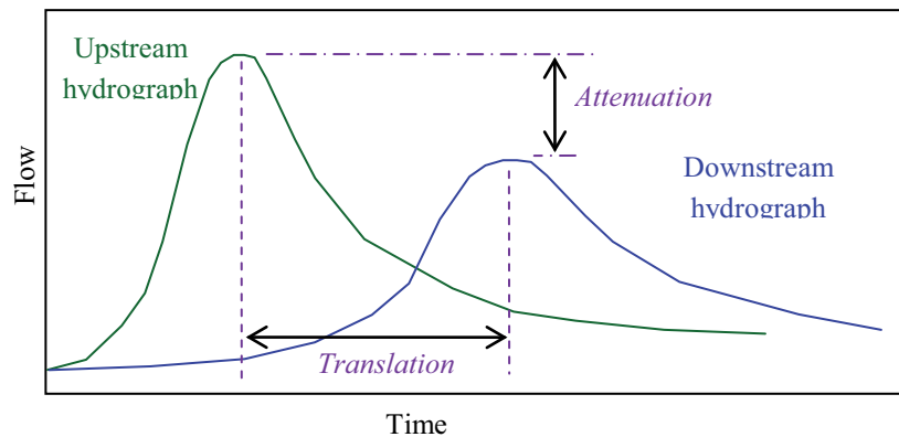
Figure 1 Flow routing
