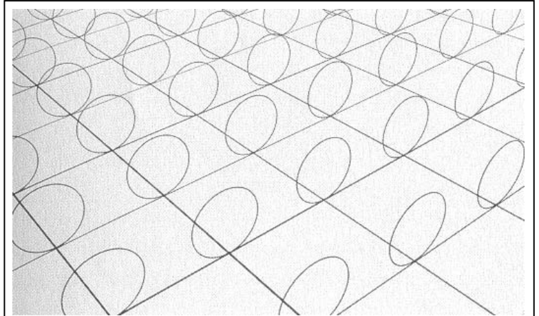
Figure 8.4 The grid lines represent the extended dimensions of common experience, whereas the circles are a new, tiny, curled-up dimension. Like the circular loops of thread making up the pile of a carpet, the circles exist at every point in the familiar extended dimensions—but for visual clarity we draw them as spread out on intersecting grid lines.
