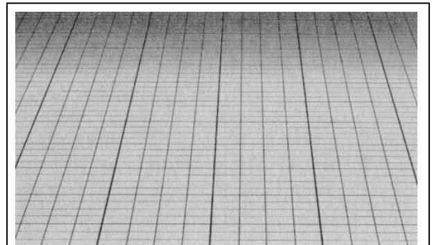
Figure 3.3 A schematic representation of flat space.
