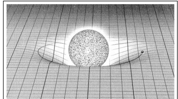
Figure 3.5 The earth is kept in orbit around the sun because it rolls along a valley in the warped spatial fabric. In more precise language, it follows a "path of least resistance" in the distorted region around the sun.
