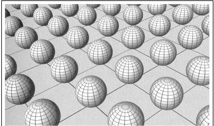
Figure 8.7 Two extra dimensions curled up into the shape of a sphere.
