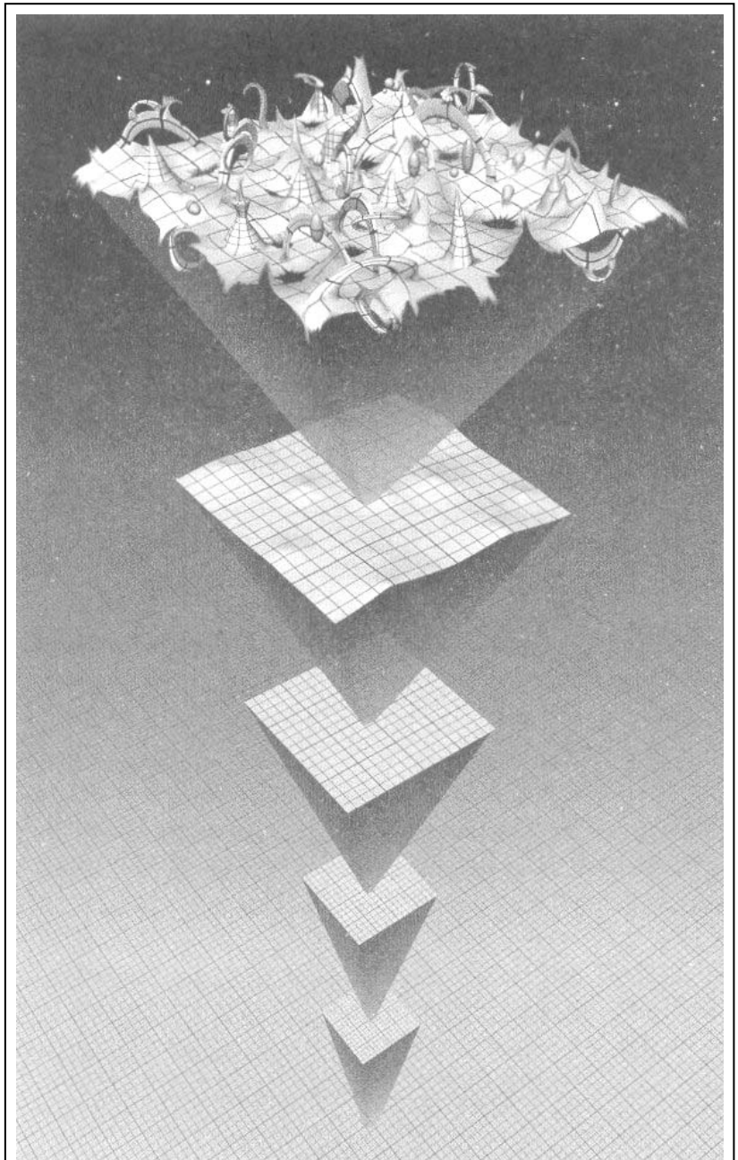
Figure 5.1 By sequentially magnifying a region of space, its ultramicroscopic properties can be probed. Attempts to merge general relativity and quantum mechanics run up against the violent quantum
