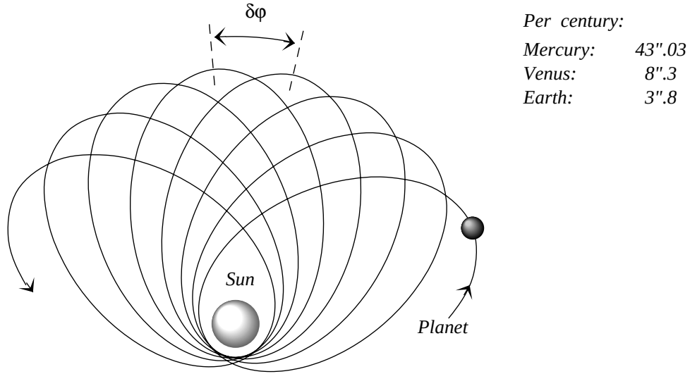
Fig.4. Perihelion shift of a planet in its orbit around a central star.
