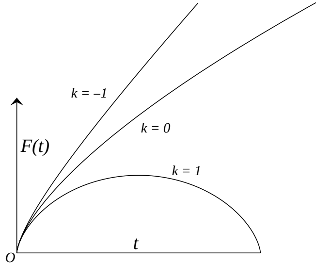
Fig. 5. The Robertson-Walker universe for k = 1 , k = 0 , and k = -1 .
