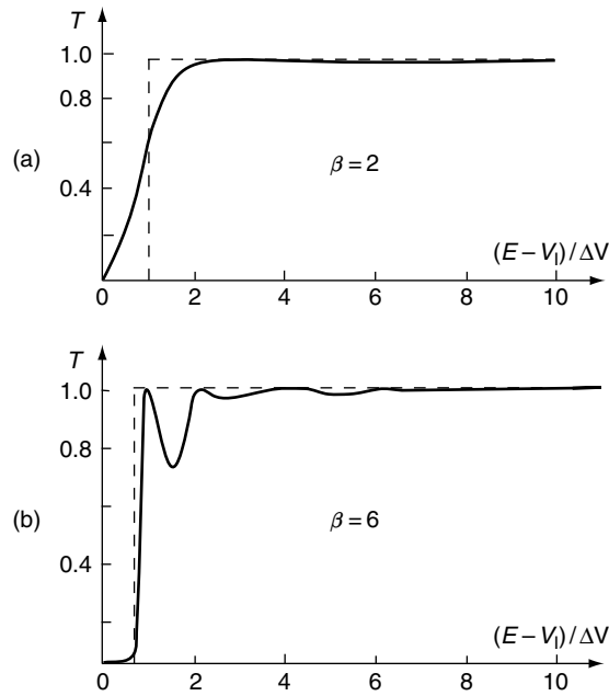
Figure 4.4. Examples of transmission curves (solid curves) of a potential barrier. (a) \beta = \sqrt{2m\Delta V d}/\hbar = 2 ; (b) \beta = 6 . The fact that T is not equal to zero for E < V_{II} corresponds to the quantum mechanical tunneling effect. The dashed lines show the classical limits.
