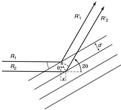
FIGURE 27.1 X-ray reflection from a set of planes.
