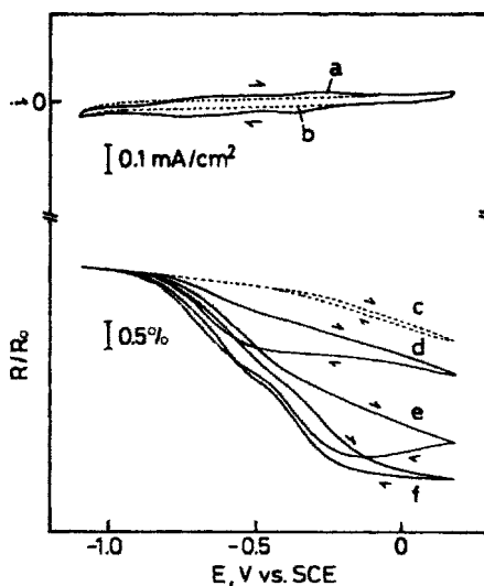
FIGURE 27.27 Cyclic voltammograms (a) and (b) and reflectivity change-potential curves (c) to (f) for 0.1 M \text{NaClO}_4 containing \text{NaI} . Concentration: (b) and (c) 0 M , (d) 5.0 \times 10^{-6} M , (e) 5.0 \times 10^{-5} M , (a) and (f) 1.0 \times 10^{-4} M . Scan rate: 0.1 \text{ V/s} . (From Arai et al., 1997, with permission from Elsevier.)
