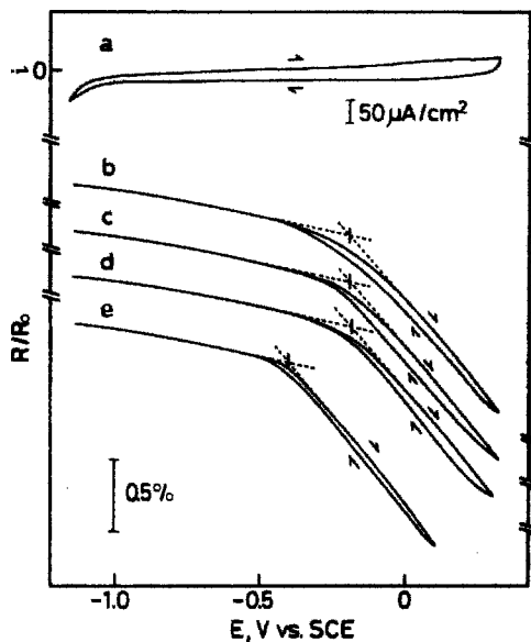
FIGURE 27.26 Cyclic voltammogram obtained on Au electrode in 0.1 M \text{NaClO}_4 (a) and reflectivity change-potential curves for 0.1 M \text{NaClO}_4 (b), 0.1 M \text{LiClO}_4 (c), 0.1 M \text{NaNO}_3 (d), and 0.1 M \text{NaOH} (e). Scan rate: 0.1 \text{ V/s} . (From Arai et al., 1997, with permission from Elsevier.)
