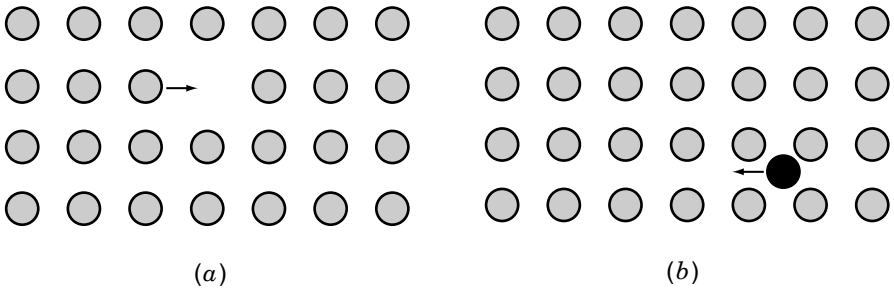
FIGURE 25.3 Schematic representation of ionic motion by (a) a vacancy mechanism and (b) an interstitial mechanism. (From Smart and Moore, 1996, Fig. 5.4, with permission from Routledge/Taylor & Francis Group.)
