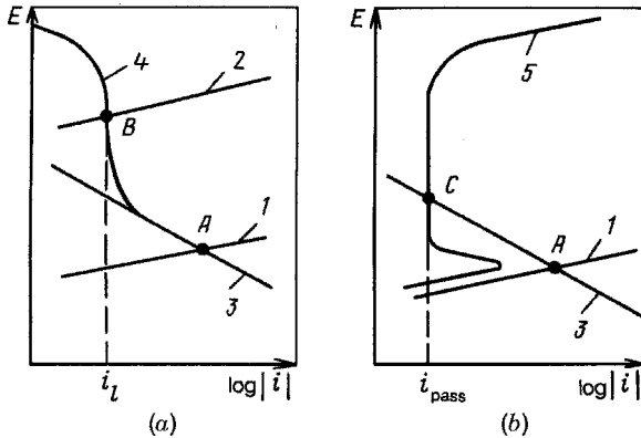
FIGURE 22.2 Schematic polarization curves for spontaneous dissolution: (a) of active metals; (b) of passivated metals. (1,2) Anodic curves for active metals; (3) cathodic curve for hydrogen evolution; (4) cathodic curve for air–oxygen reduction; (5) anodic curve of the passivated metal.
