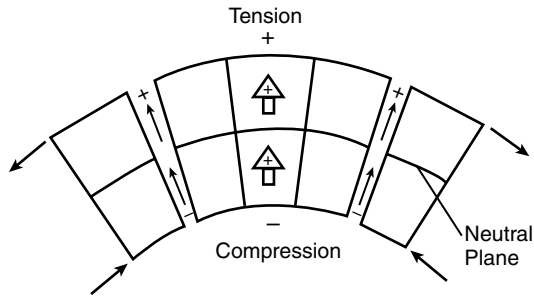
FIGURE 24.1 Surface potentials generated by bending of bone.
