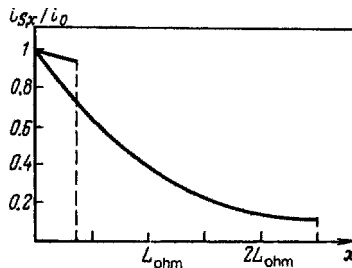
FIGURE 18.5 Current density distribution inside a porous electrode [according to Eq. (18.18)] for two values of electrode thickness: d_1 = 0.33L_{\text{ohm}} and d_2 = 2.5L_{\text{ohm}} .
