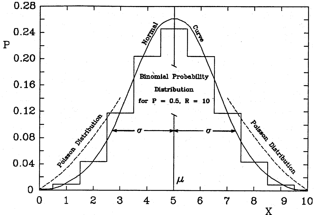
Figure 7.2 shows the normal curve approximation to the binomial probability distribution function. We have chosen the coin tosses so that p = 0.5 . Here \mu and \sigma can be seen as the most likely value of the random variable x and the 'width' of the curve respectively. The tail end of the curve represents the region approximated by the Poisson distribution.
