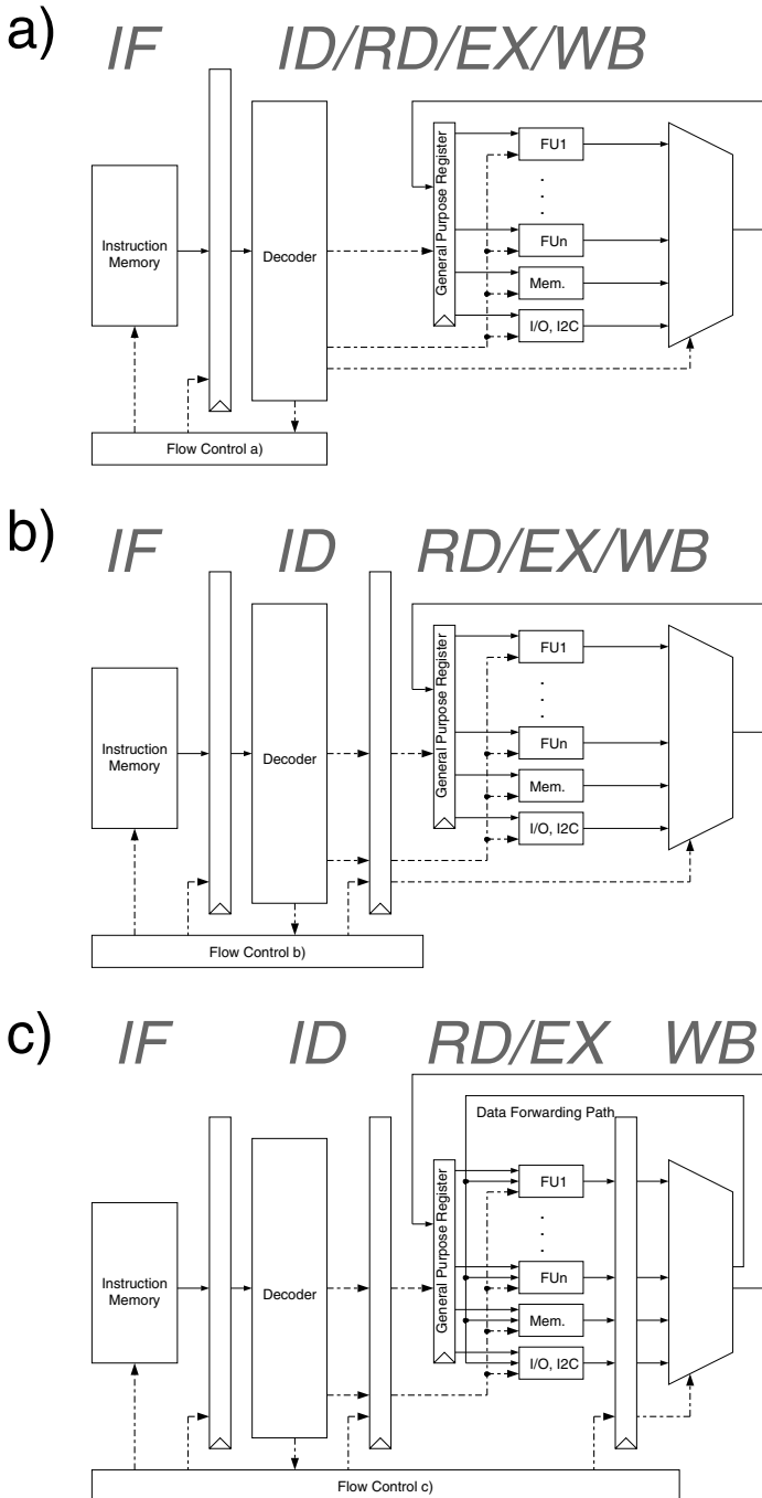
Figure D.1: Different Pipeline Organizations for Design Exploration
