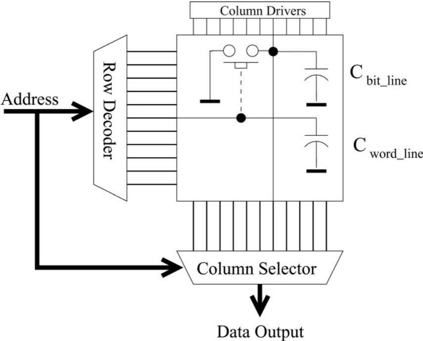
Figure 6.6: ROM Model with Capacitances
