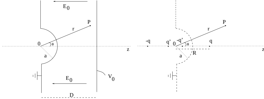
Figure 2.5: On the left is the geometry of the problem: two conducting plates separated by a distance D . One of the plates has a hemispheric boss of radius a . The electric field between the two plates is E_0 . On the right is the set of charges that image the field due to the conducting plates. In part a and b, R \rightarrow \infty to image a homogeneous field. In c, R = d .
