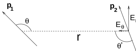
Figure 3.1: Coplanar dipoles separated by a distance r .
