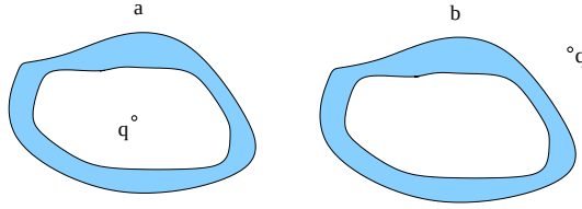
Figure 1.1: a: point charge in the cavity of a hollow conductor. b: point charge outside the cavity of a hollow conductor.
