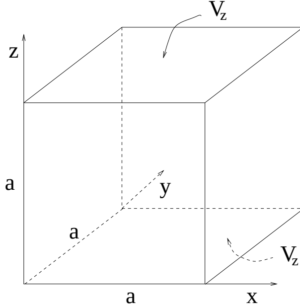
Figure 2.9: A hollow cube, with all sides but z=0 and z=a grounded.
