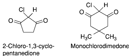
FIG. 2. Chemical structure of 2-chloro-1,3-cyclopentanedione, an intermediate in caldariomycin biosynthesis and the synthetic compound monochlorodimedone, which was used in the search for haloperoxidases.
