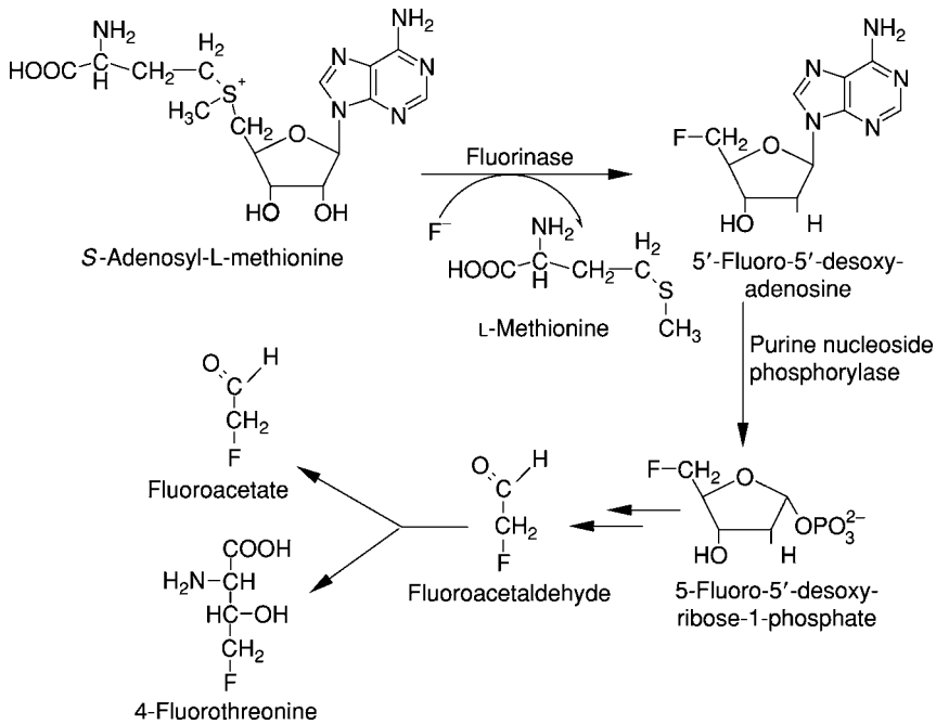
FIG. 12. The fluorinase reaction leading to the formation of 5'-fluoro-5'-desoxyadenosine from S -adenosyl-L-methionine as the substrate and further metabolization of 5'-fluoro-5'-desoxyadenosine to fluoroacetate and 4-fluorothreonine.
