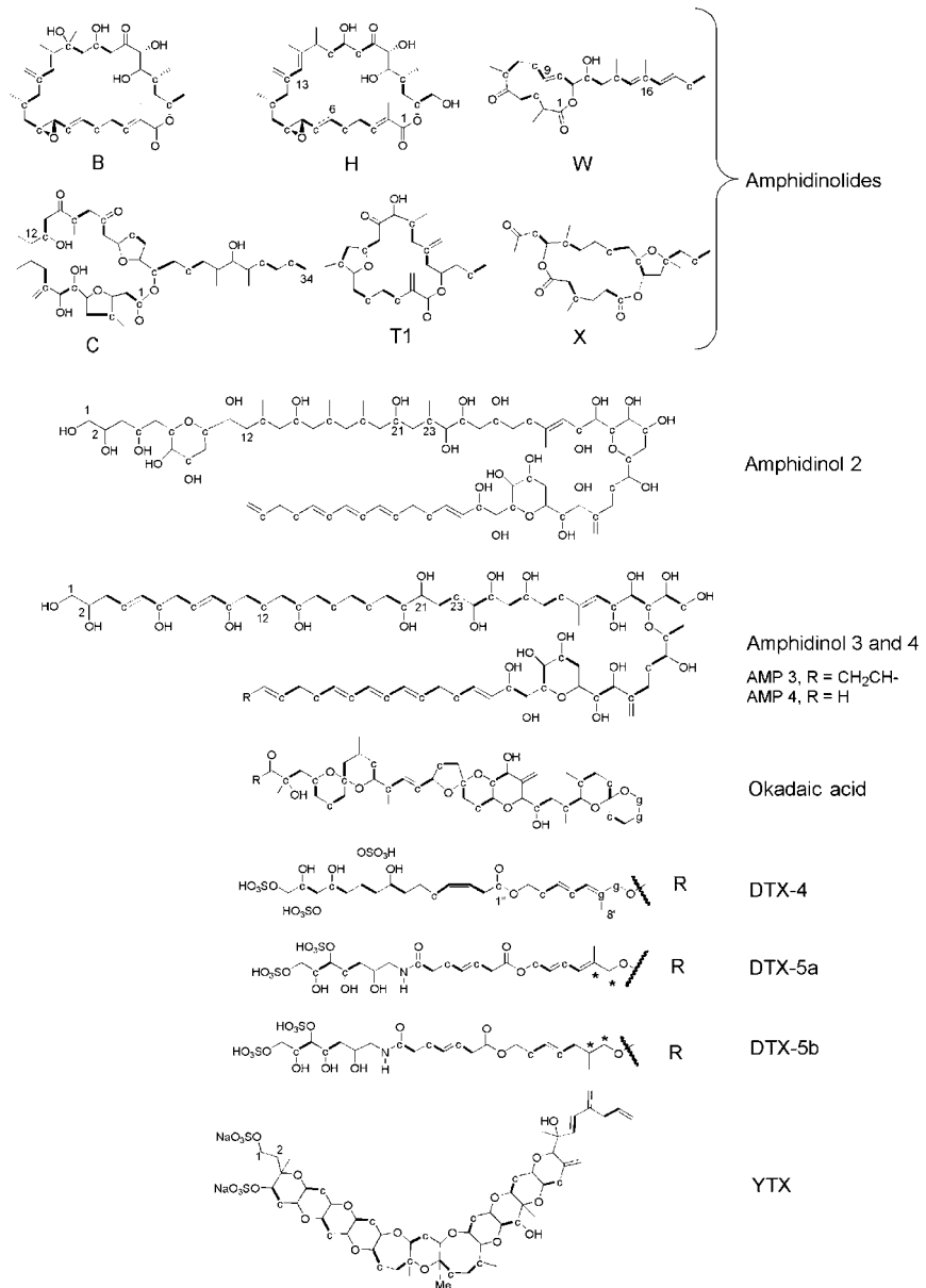
FIG. 5. Labeling pattern of polyketides from stable isotope feeding experiments including amphidinolides, amphidinols, okadaic acid and dinophysins toxins, and yessotoxin. Legend: g = glycolate, c = C1 acetate, m = C2 acetate, Me represents methyl
