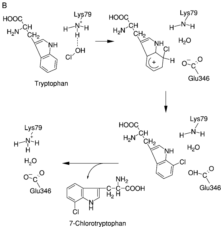
FIG. 10. Proposed reaction mechanism of flavin-dependent halogenases. (A) In the first part of the reaction FAD is reduced to FADH 2 by a flavin reductase. (B) In the second part of the reaction HOCl is formed at the active site of the enzyme and is guided by interaction with lysine 79 to the correct position at the substrate tryptophan. Flavin blocks the entrance to the tunnel thus preventing HOCl from leaving the active site.
