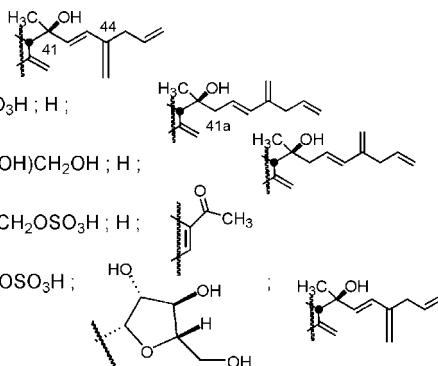
FIG. 2. Novel polyketides from dinoflagellates. See text for details.
