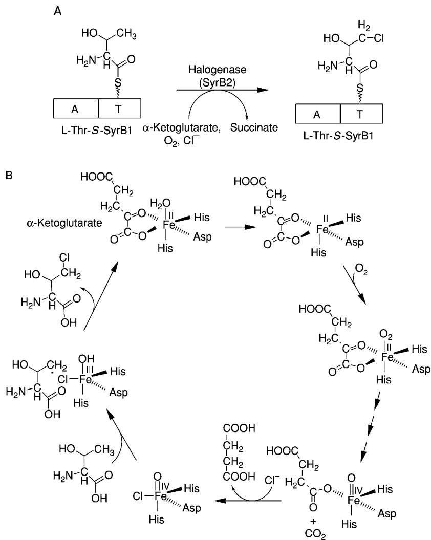
FIG. 11. Chlorination of a nonactivated alkyl group by a nonheme \text{Fe}^{\text{II}} , \alpha -ketoglutarate- and oxygen-dependent halogenase. (A) Previous to halogenation, the substrate is bound to a thiolation domain. (B) In the suggested mechanism, a substrate radical is formed which attacks the chlorine bound to the nonheme iron.
