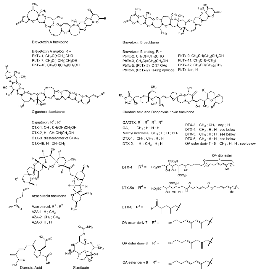
FIG. 1. Marine algal toxins responsible for classified human illnesses. Also shown are ester derivatives of okadaic acid.
