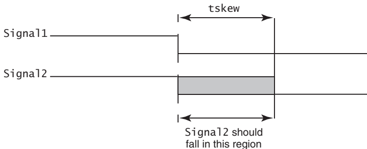
Figure 8.7 In-phase skew check
