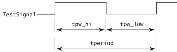
Figure 8.3 Period/pulsewidth check
