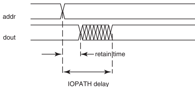
Figure 4.3 Retain time
