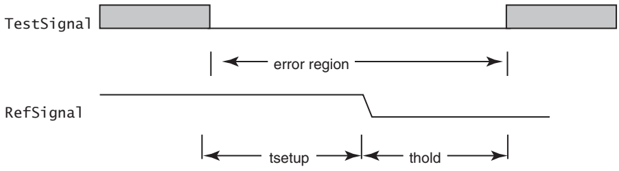
Figure 8.1 Setup/hold check
