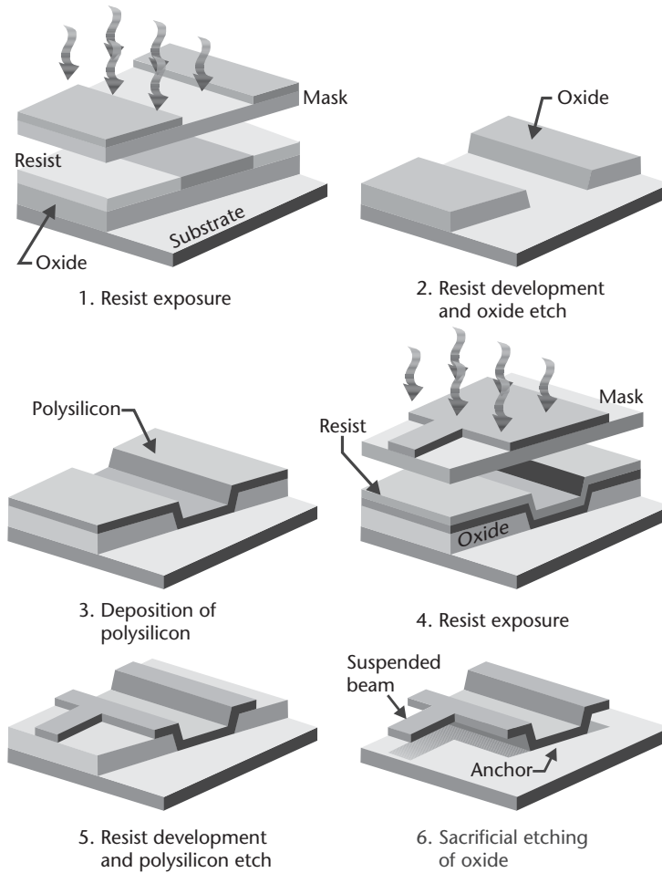
Figure 3.29 Schematic illustration of the basic process steps in surface micromachining.
